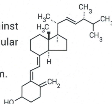
Chemical Formula
